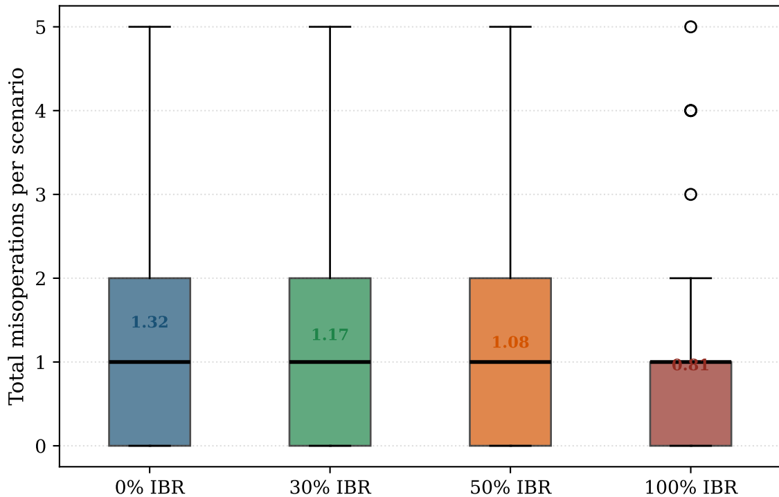
Total SAMBP misoperations per N-2 scenario IEEE 118-bus, 100 scenarios per IBR level
