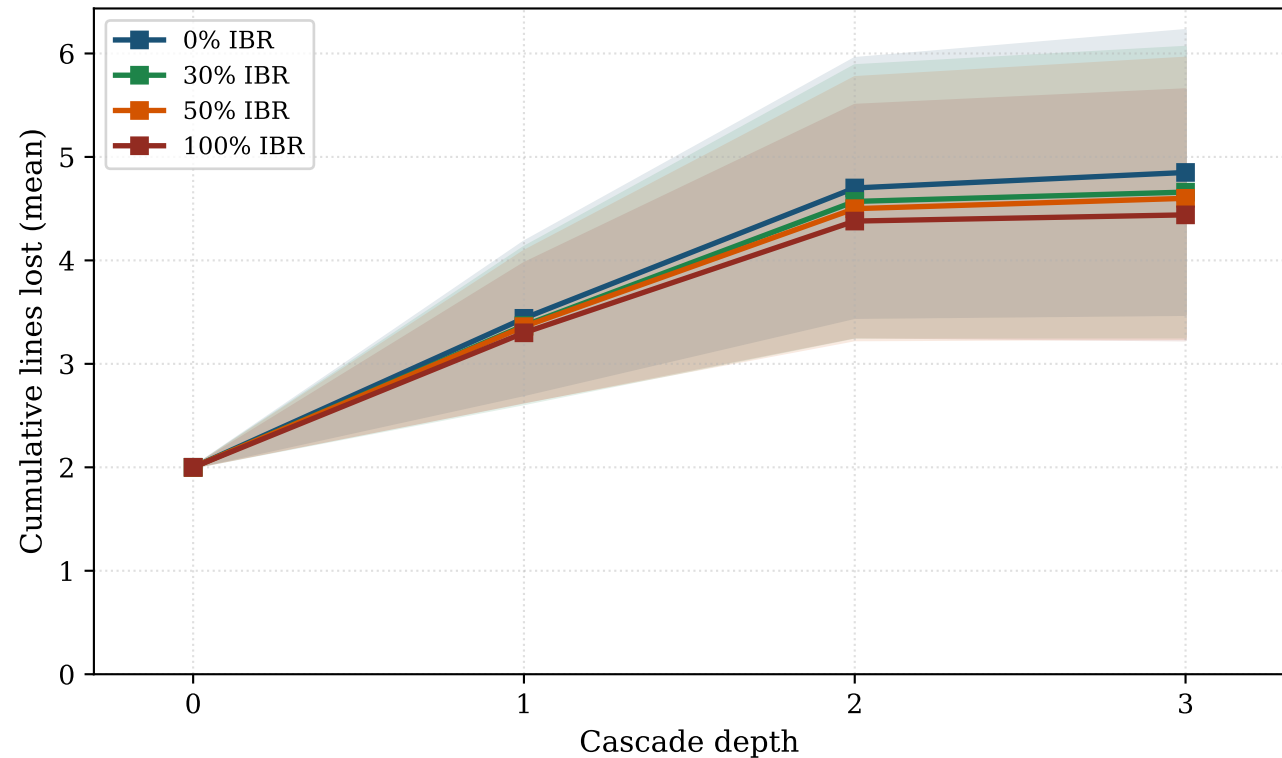
Cumulative lines lost vs cascade depth Mean \pm 1\sigma across 100 N-2 scenarios
