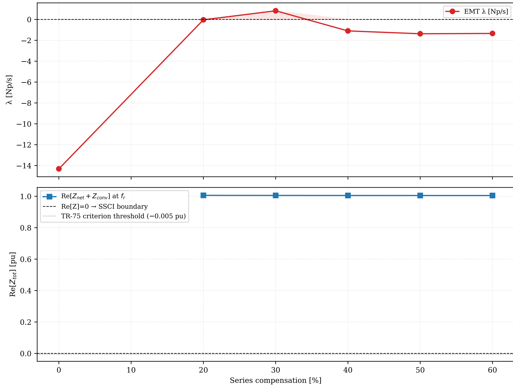
TR-75: EMT Growth Rate vs Impedance Criterion Comparison
