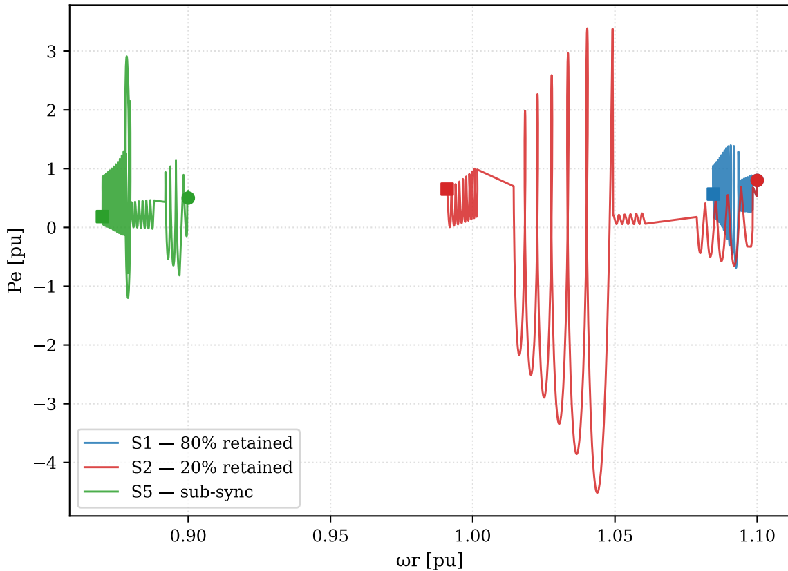
DFIG EMT — Phase Portrait: P_e vs \omega_r Circle = start, square = end of simulation
