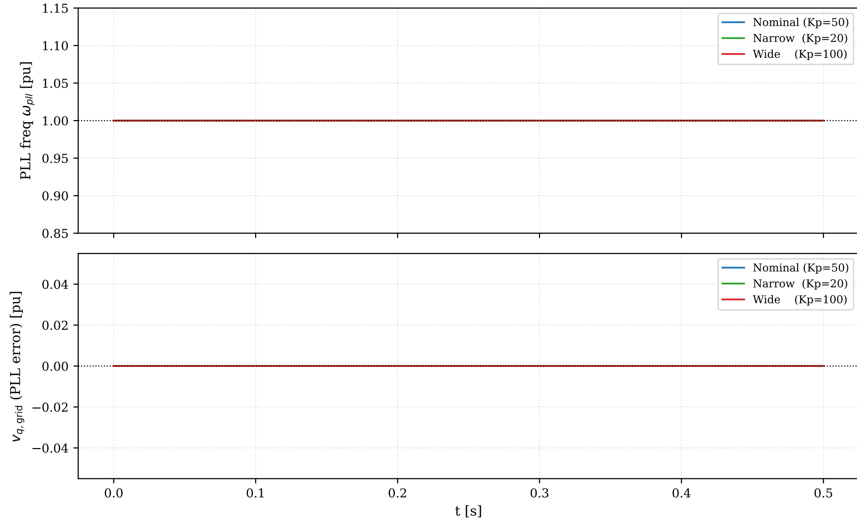
PV Inverter EMT — PLL Bandwidth Comparison under 50% Dip S1 (nominal), narrow PLL ( K_p=20 ), wide PLL ( K_p=100 )
