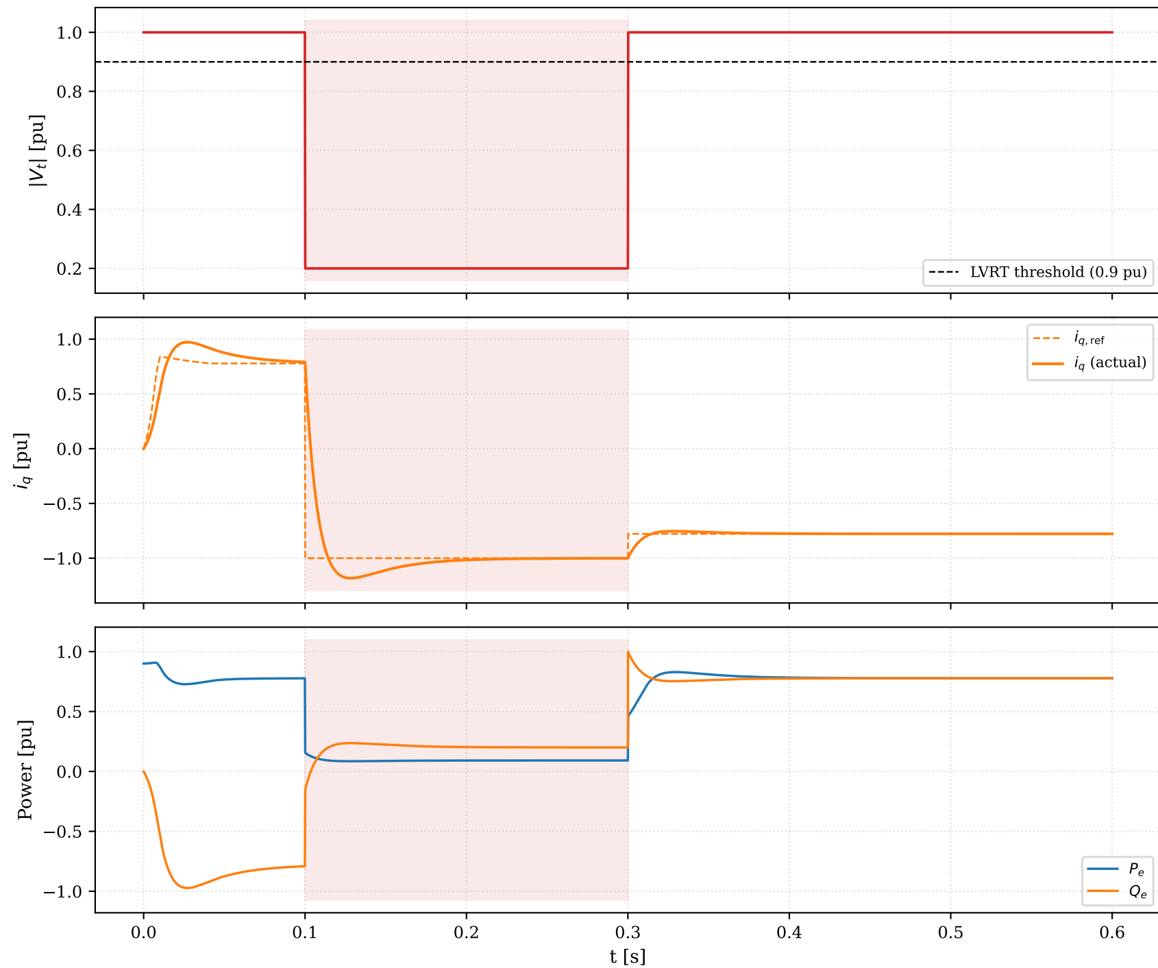
PV Inverter EMT — LVRT Reactive Current Injection S2: 20% retained dip; reactive priority per IEC 61400-21
