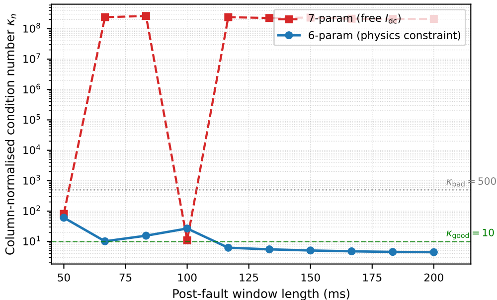
Estimator ill-conditioning vs window length
