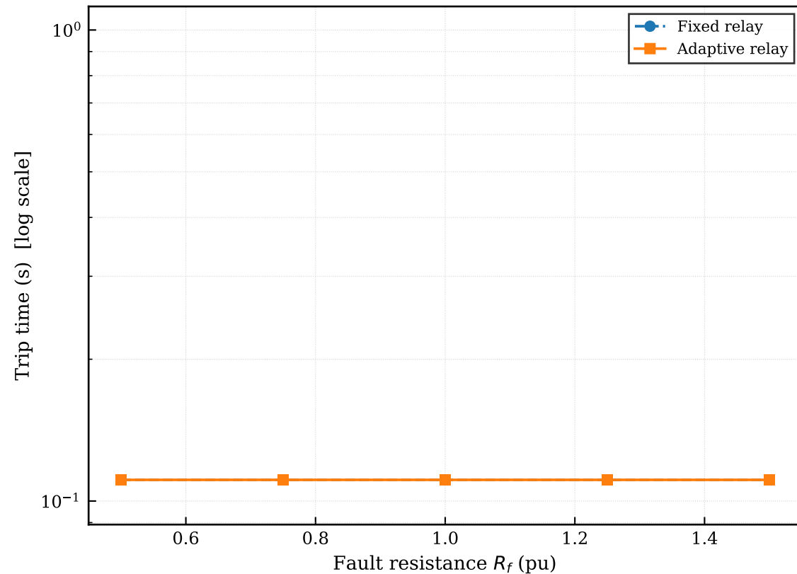
HIF trip time vs R_f — SLG
