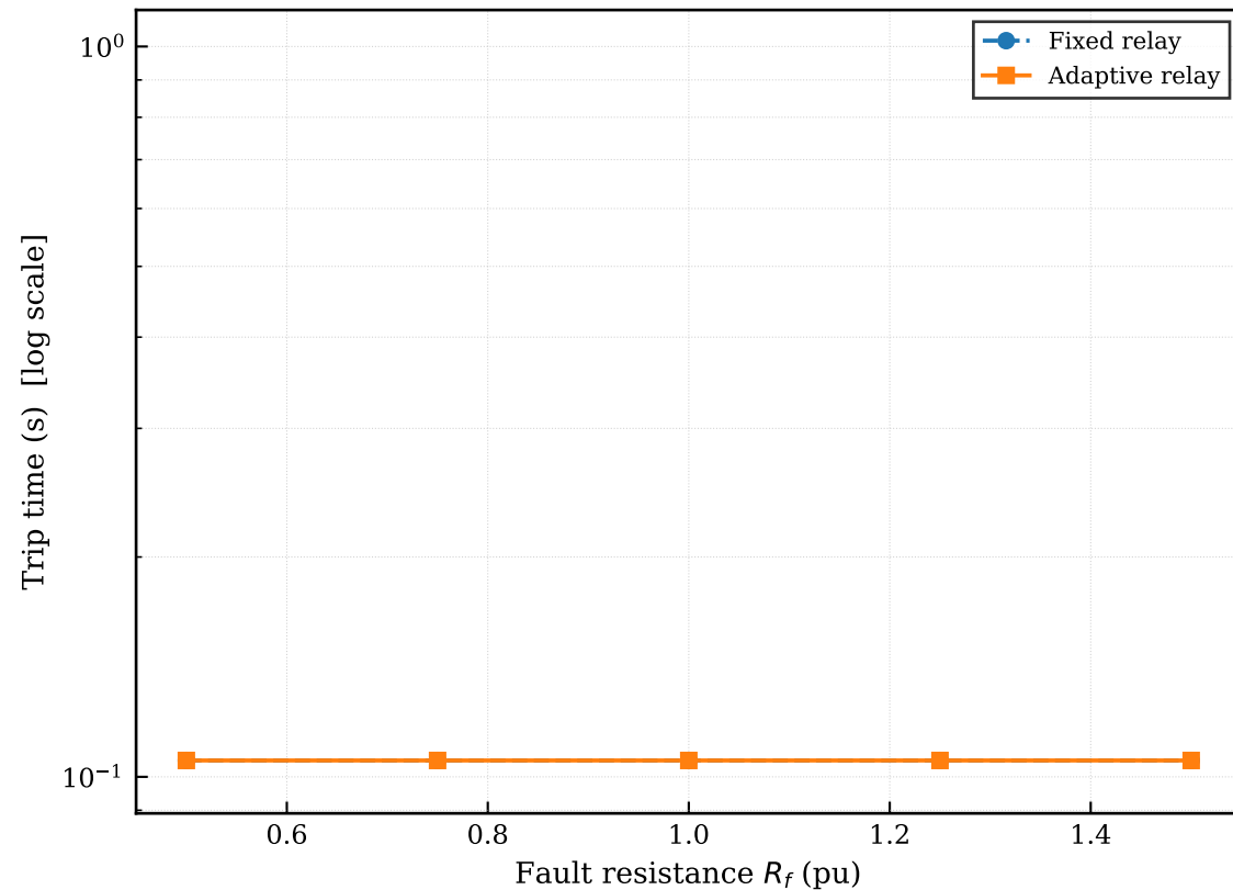
HIF trip time vs R_f — 3PH
