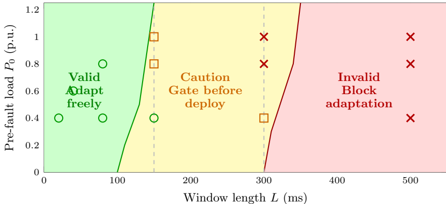
Relay-validity map: reduced inverse model under 6th-order dynamics
