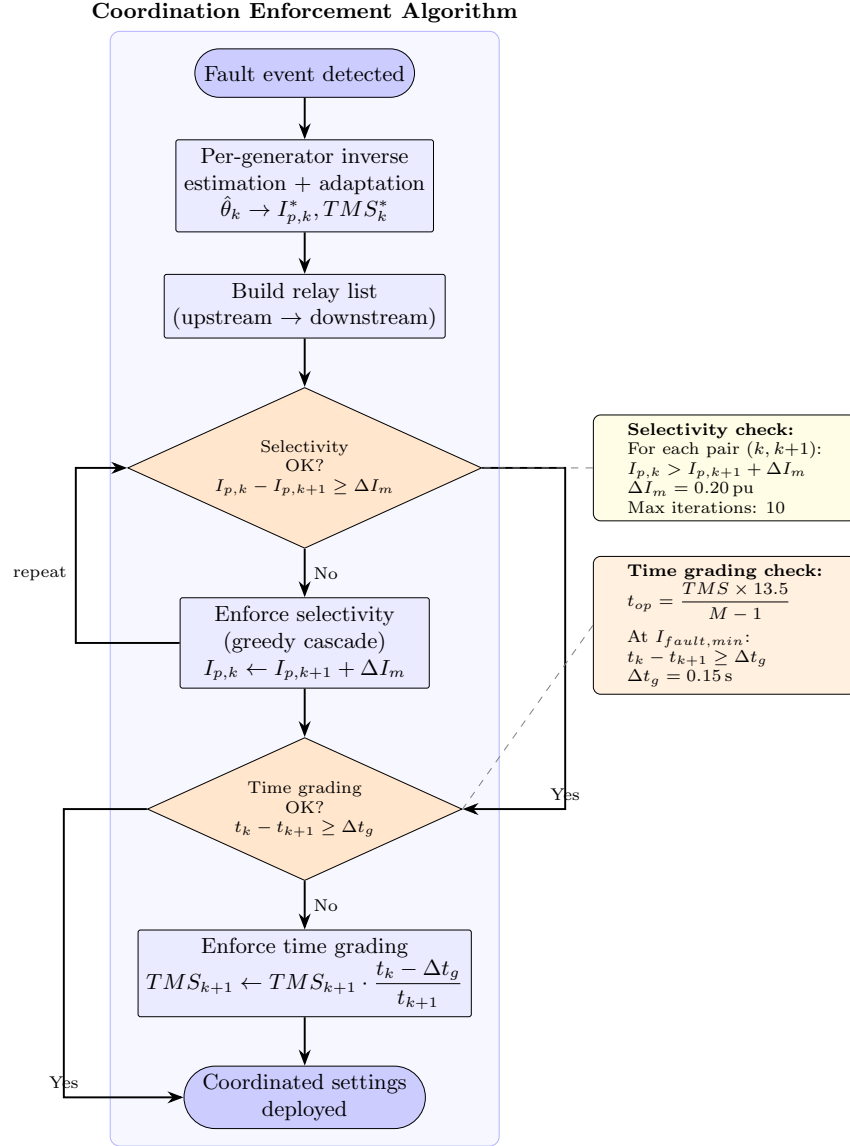
Figure 5: Coordination enforcement flowchart. After per-generator adaptive estimation and mapping, selectivity (eq. (31)) is checked and enforced by the greedy cascade algorithm, followed by trip-time grading (eq. (32)) enforcement via minimal TMS reduction. Both checks converge within 10 iterations for the study system.
