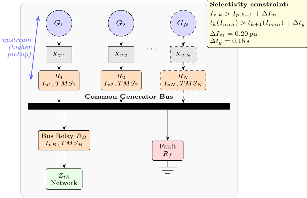
Figure 4: Multi-generator busbar system. Each generator G_k is connected to the common bus through a step-up transformer X_{T_k} and a generator relay R_k . The bus relay R_B is downstream of all generator relays. The selectivity constraint (yellow box) requires each upstream relay to have a higher pickup than the relay downstream of it.
