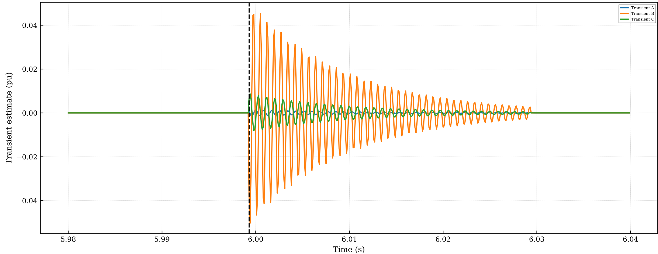
Reduced-Order Transient Model
