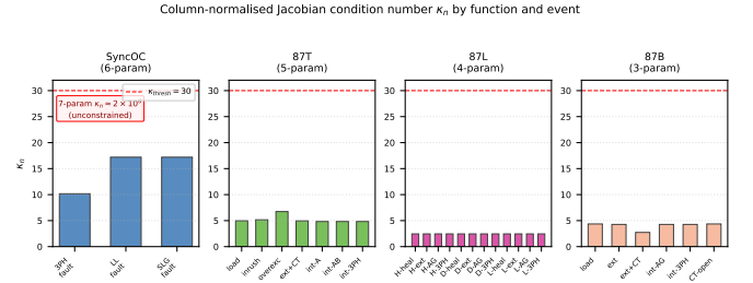
Fig. 5: Column-normalised Jacobian condition number \kappa_n for all 28 simulation scenarios grouped by protection function. Red dashed line: \kappa_{thresh} = 30 . All constrained models remain well below threshold. The unconstrained SyncOC 7-parameter model ( \kappa_n \approx 2 \times 10^8 , shown as annotation) demonstrates the necessity of the physics-reduction step.
