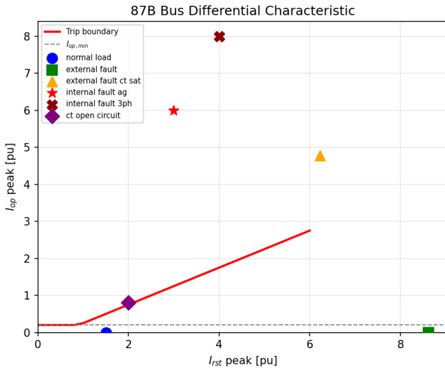
Fig. 4: 87B differential characteristic with 6 test events overlaid. Normal load and external fault lie in the no-trip region (conv_trip = 0). External fault + CT saturation is intercepted by the model veto. Internal AG and 3PH faults trip conventionally. CT open-circuit is an architectural boundary case (see §VI-C).
