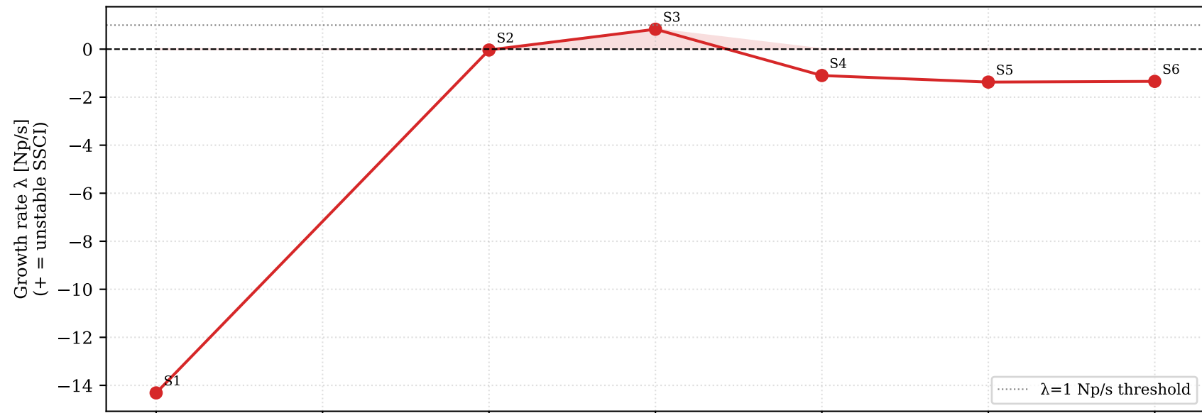
TR-75 DFIG SSCI — EMT Growth Rate vs Series Compensation
