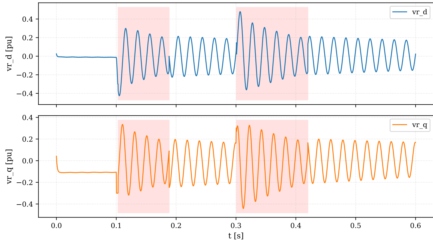
DFIG EMT — RSC Voltage Commands during Deep Dip (S2) Red shading: crowbar active, RSC blocked
