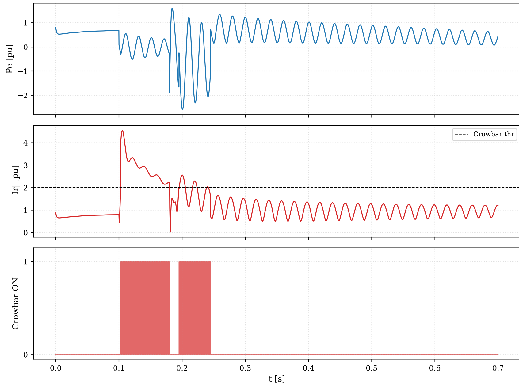
DFIG EMT — S4 Crowbar Cycling under Repeated Dip
