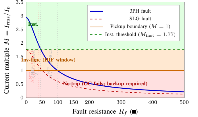
Fig. 2. Operating-regime map: current multiple M vs R_f for 3PH (solid blue) and SLG (dashed red) faults. The three regimes (instantaneous, inverse-time HIF window, no-trip) are shaded in green, orange, and red respectively. Regime boundaries for the study system are R_f^{\text{HIF}} = 46 \Omega and R_f^{\text{NT}} = 98 \Omega (3PH); the SLG window closes earlier due to reduced fault current.
