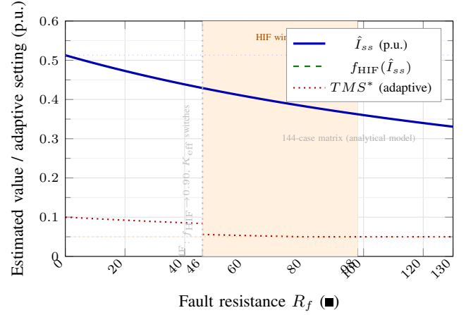
Fig. 7. Estimated \hat{I}_{ss} , correction factor f_{\text{HIF}} , and adaptive TMS TMS^* vs. R_f . At the HIF boundary ( R_f \approx 46 \Omega ), f_{\text{HIF}} drops below 0.90 and K_{\text{TMS}}^{\text{eff}} switches from 0.12 to 0.08. For deep HIF ( R_f > 90 \Omega ), TMS^* clips to TMS_{\min} = 0.05 . Results consistent with 144-case matrix; analytical curves validated.
