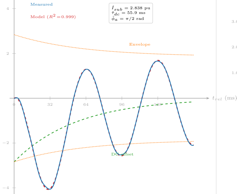
(a) Phase-A waveform fit
