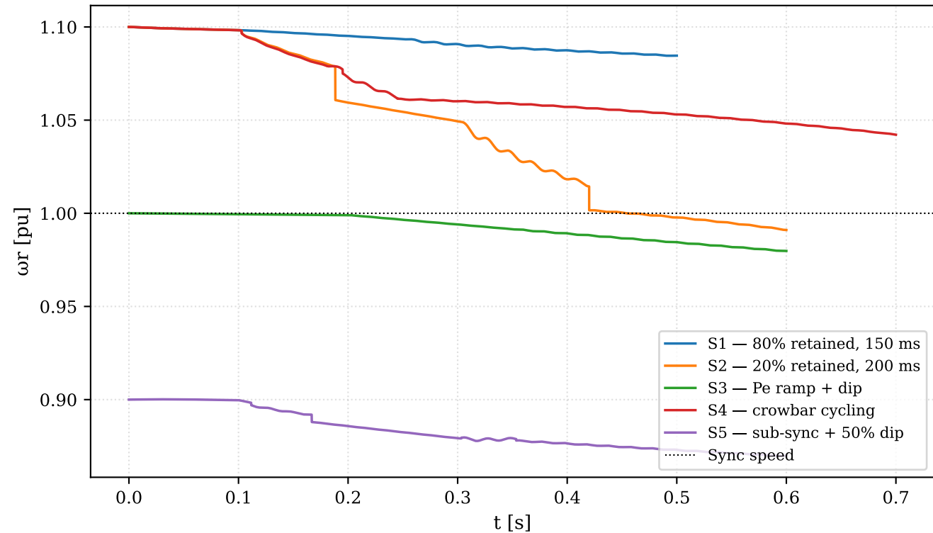
DFIG EMT — Rotor Speed Dynamics All 5 scenarios
