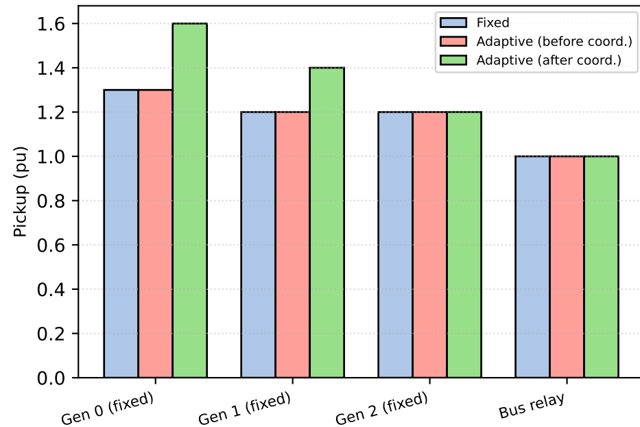
Relay Pickup Settings
