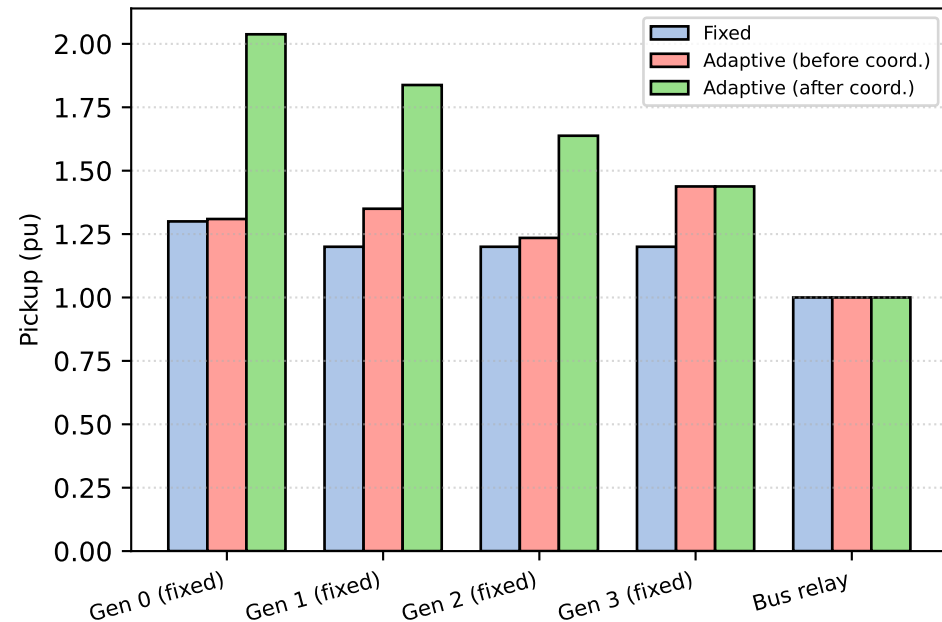
Relay Pickup Settings
