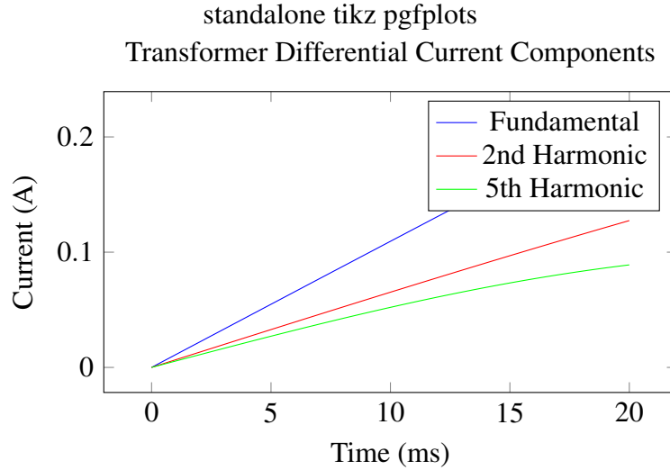
Figure 2: Components of transformer differential current.
