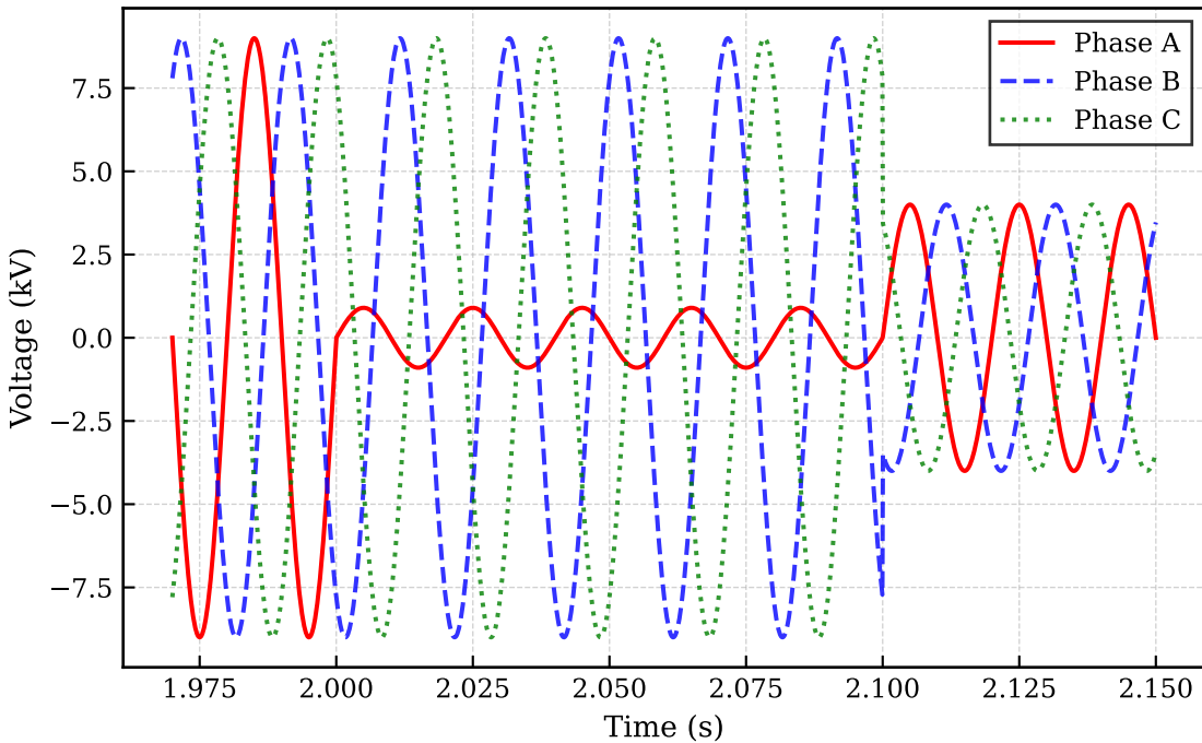
Three-Phase Voltage Waveform: Multi-Stage Voltage Dip
