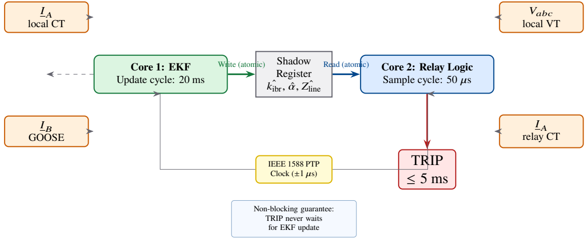
Figure 9.1: Non-blocking digital twin architecture. The EKF runs on a dedicated processing core at 20 ms cycle time. The relay protection logic on a separate core reads the latest EKF estimate from the shadow register at every 50 \mu s sample. GOOSE messages from adjacent relays supplement the local current measurements.
