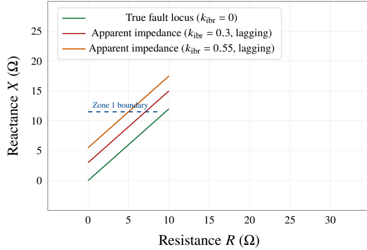
Figure 7.1: Apparent impedance locus for faults at \alpha \in [0, 1] with fault resistance R_F = 10 \Omega . The classical mho Zone 1 boundary is shown. For k_{ibr} = 0.55 with lagging reactive injection ( \beta = -90^\circ ), faults at \alpha > 0.85 enter Zone 1, causing overreach.
