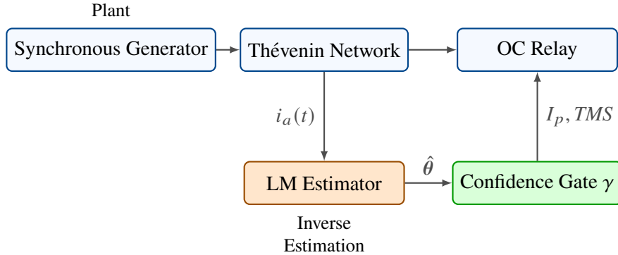
Figure 5.1: SAMBP-SyncOC study system. The physical plant (SG + Thevenin network) provides three-phase current measurements to the inverse estimation and adaptation layer. The LM estimator feeds the confidence scorer; the bounded update law ensures relay settings remain within safe operational bounds.
