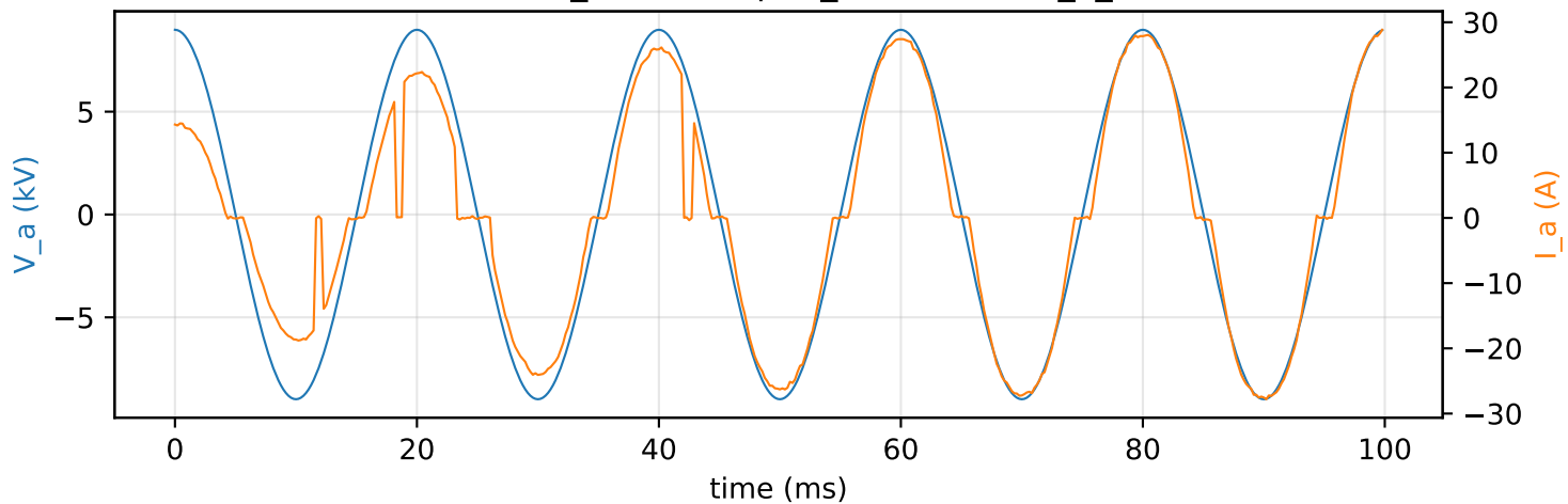
Scenario 26 (torres_tree) — \alpha_{\text{true}}=0.10 , R_{\text{x\_true}}=200\ \Omega
