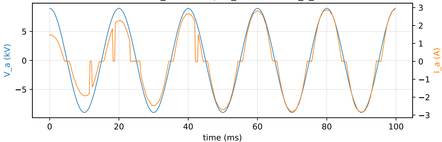
Scenario 29 (torres_tree) — \alpha_{\text{true}}=0.70 , R_{\text{x\_true}}=2000 \Omega
