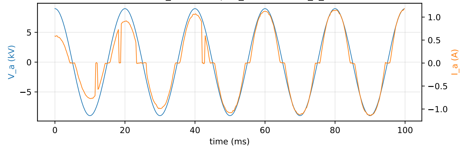
Scenario 30 (torres_tree) — \alpha_{\text{true}}=0.90 , R_{x\_true}=5000\ \Omega
