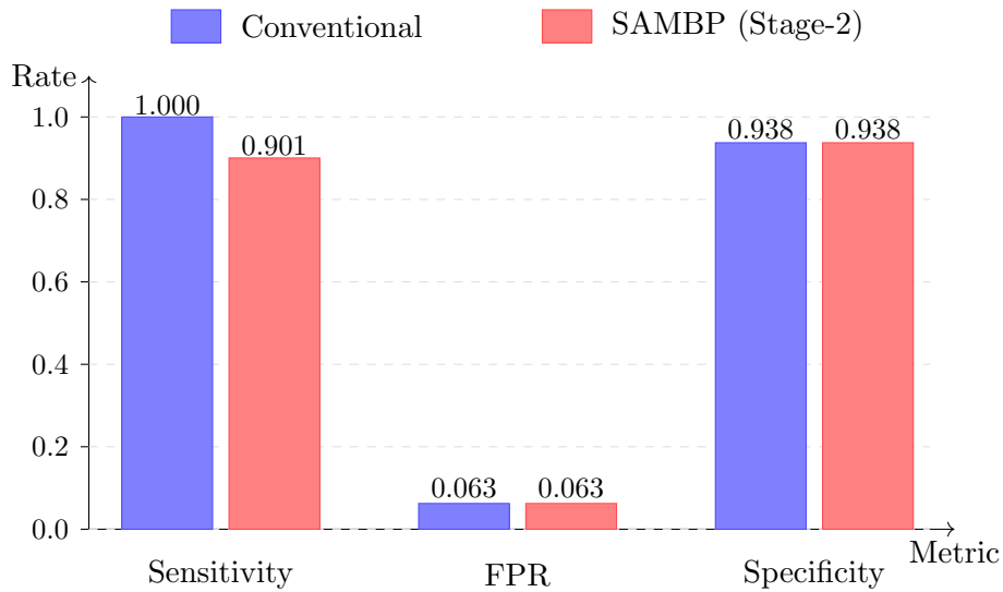
Figure 2: Aggregate performance comparison. Conventional (blue) vs. SAMBP Stage-2 (red). Both methods share identical FPR and specificity; the SAMBP sensitivity shortfall is concentrated in three-phase bus differential scenarios.
