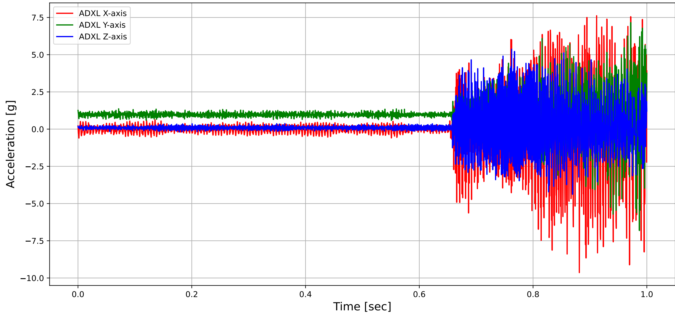
ADXL Accelerometer Data
