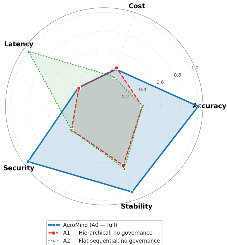
Figure 3: Figure 3 — Measured CLASSic ablation: AeroMind (A0) vs governance-ablated hierarchical (A1) vs flat sequential (A2)
