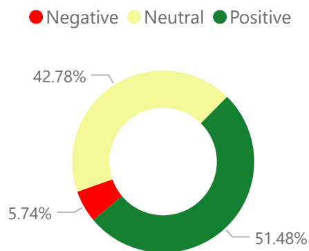
Sentiment Distribution
