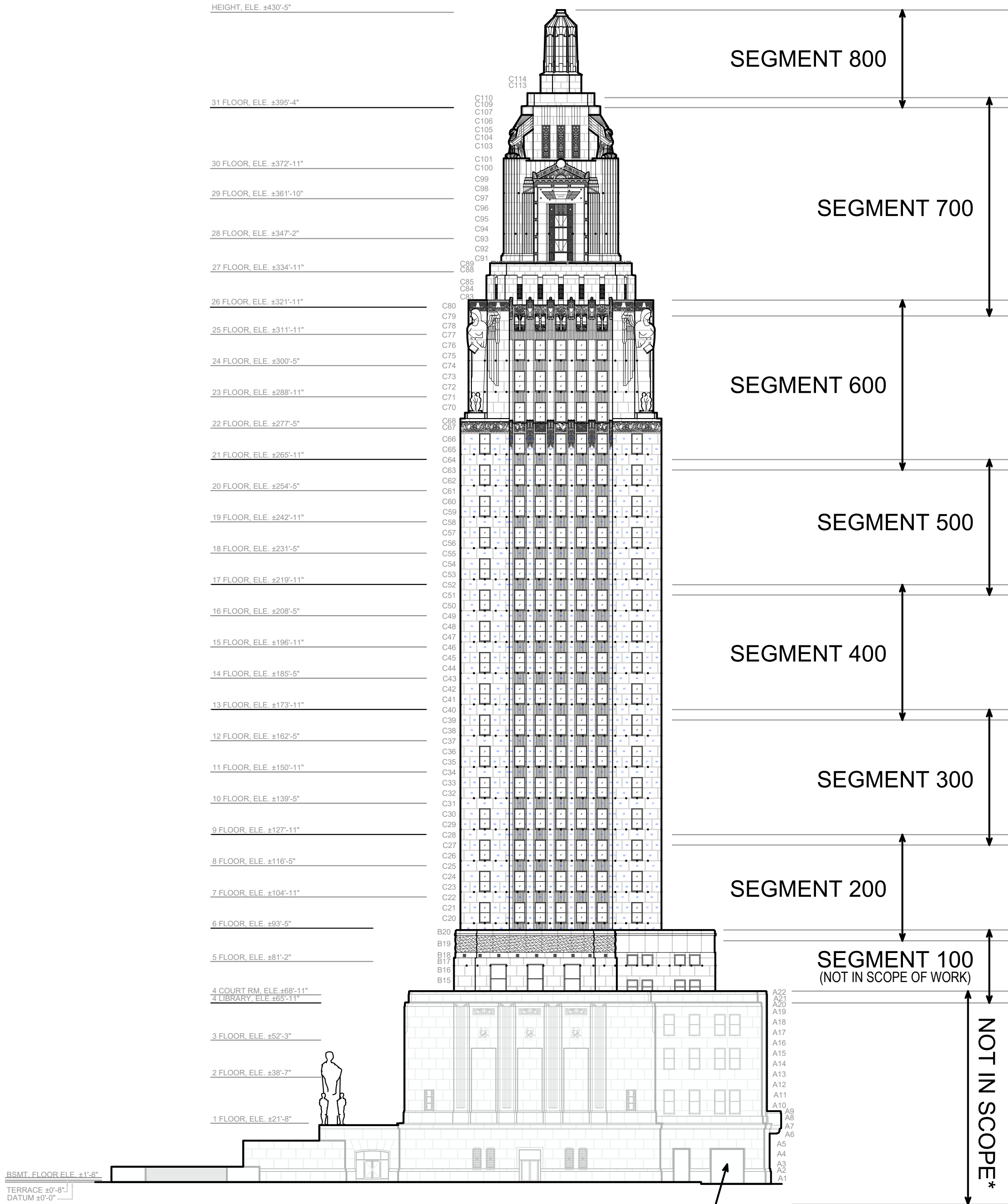
2 EAST KEY ELEVATION SCALE: 1/4"=1'-0"
