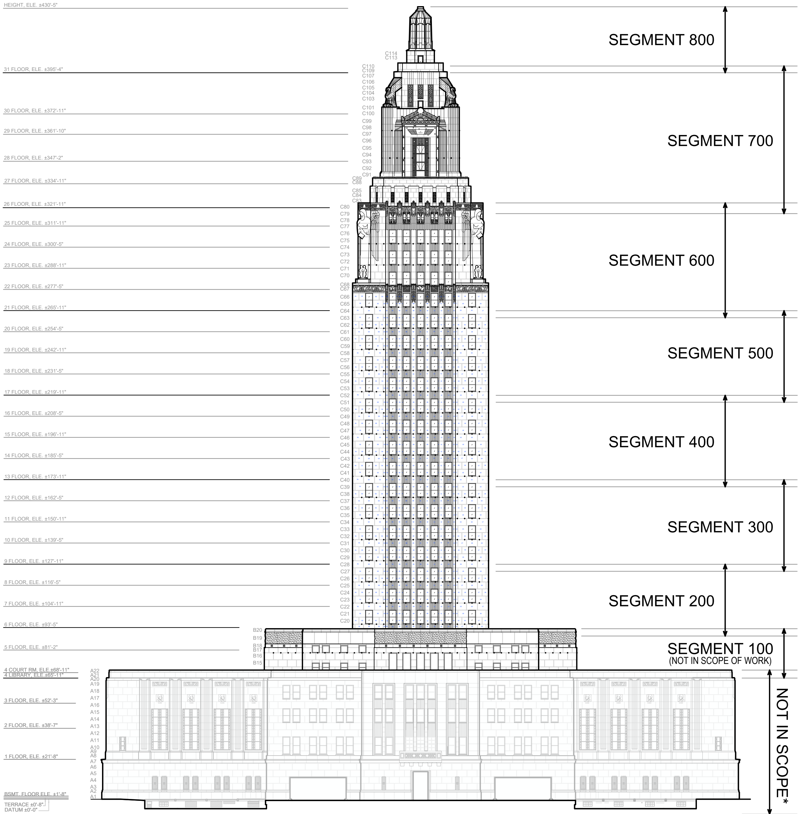
1 NORTH KEY ELEVATION SCALE: 1/32"=1'-0"
