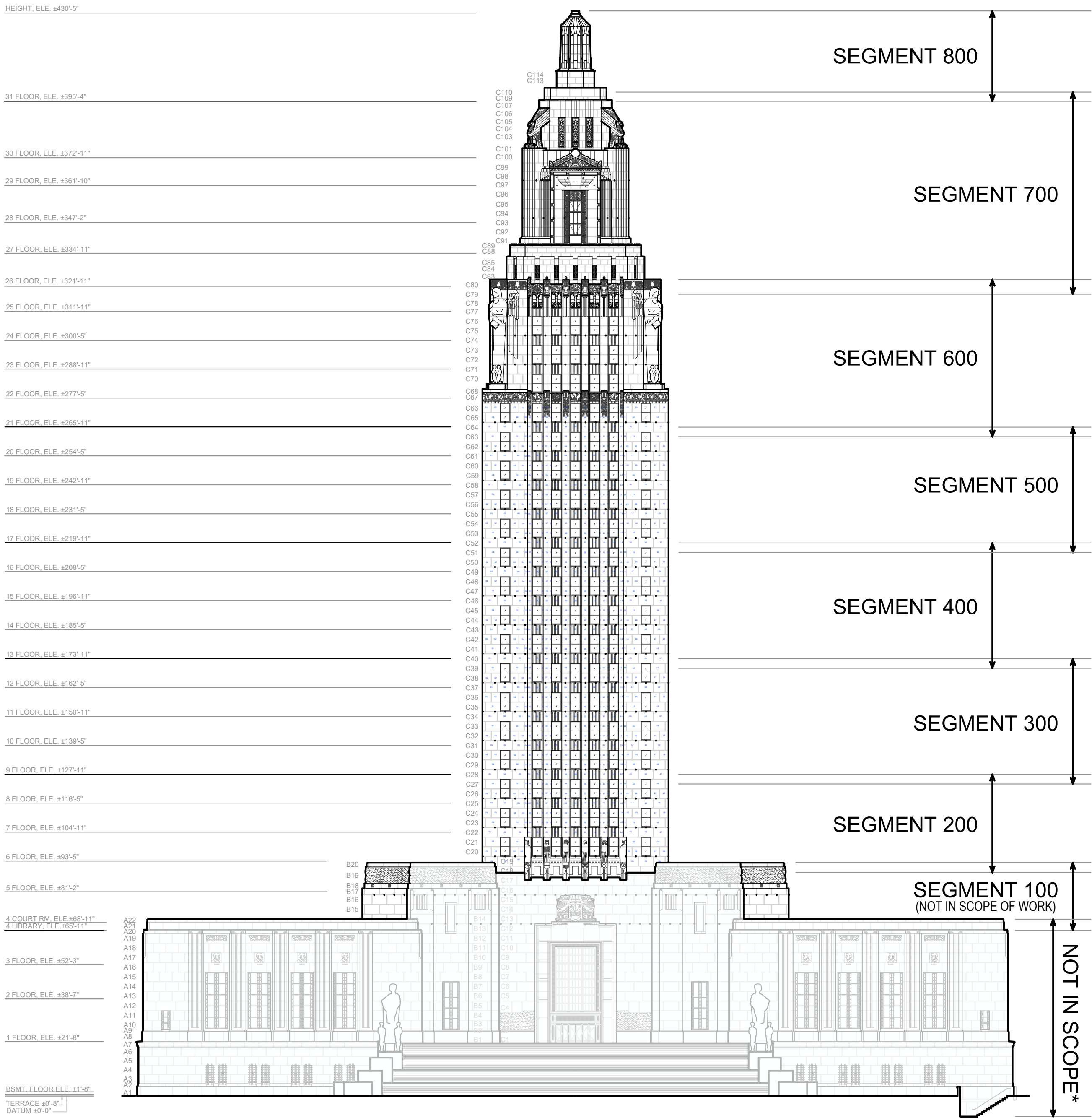
1 SOUTH KEY ELEVATION SCALE: 1/32"=1'-0"
