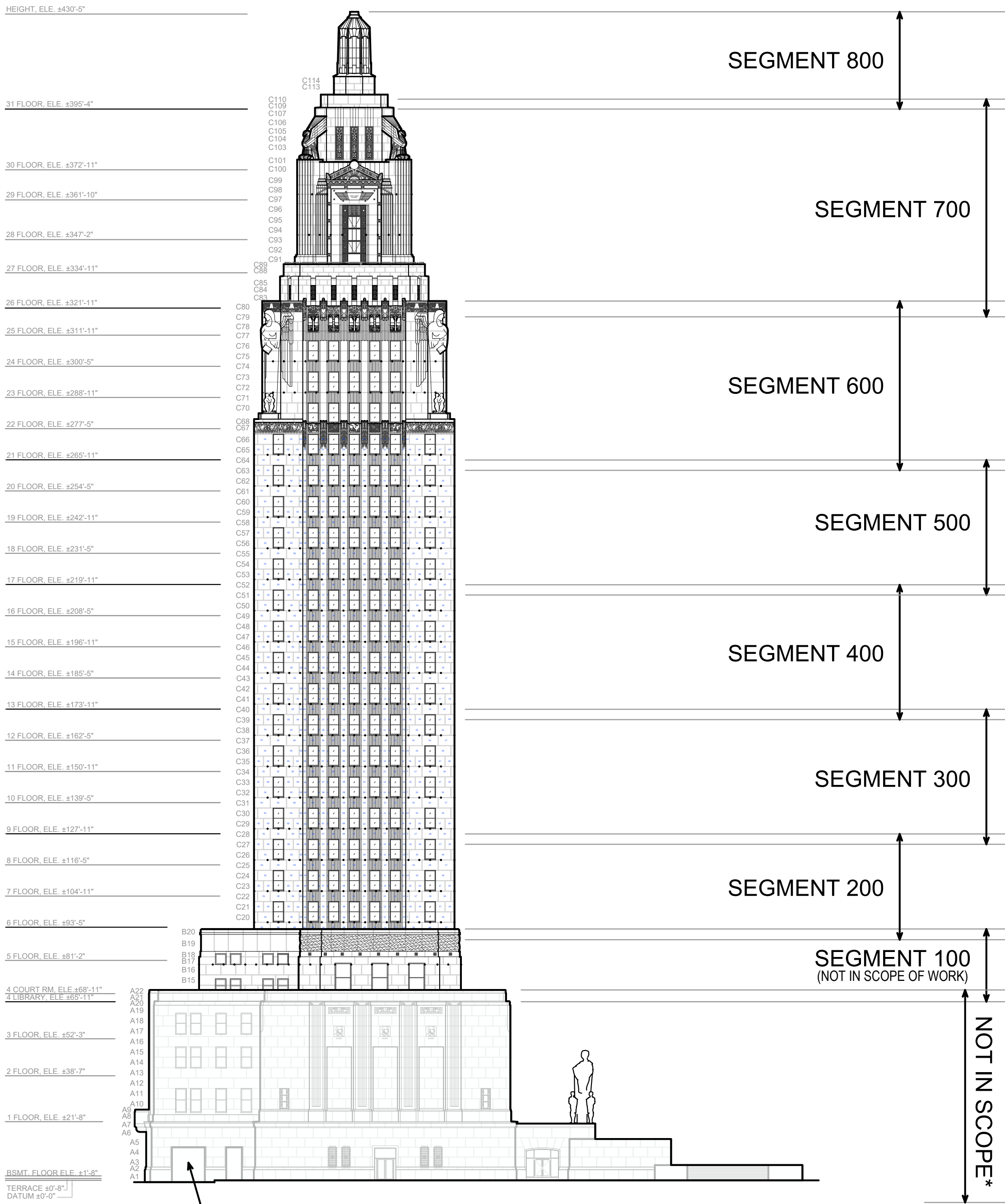
2 WEST KEY ELEVATION SCALE: 1/4"=1'-0"
