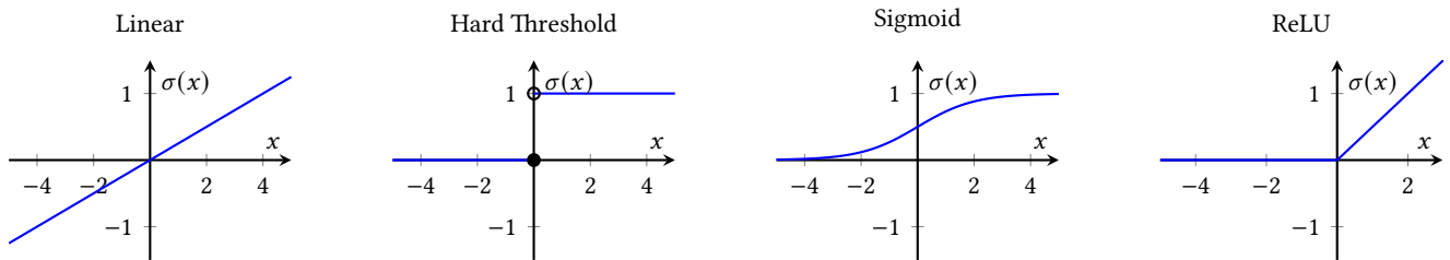
Figure 7.1: Activation functions
