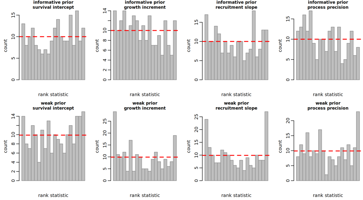
Figure 3: Simulation-based calibration rank histograms (dashed line: uniform expectation). Top: informative prior, ranks approximately uniform. Bottom: diffuse prior, U-shaped ranks indicating overconfident intervals, worst for the recruitment slope.
