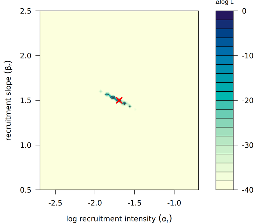
Figure 1: Relative profile log-likelihood over recruitment level \alpha_r and slope \beta_r , all other parameters at truth (red cross), capped at \Delta \log L = -40 to reveal structure. The likelihood is sharply peaked except along a thin ridge oriented in the negative-correlation direction: the non-identified recruitment direction.
