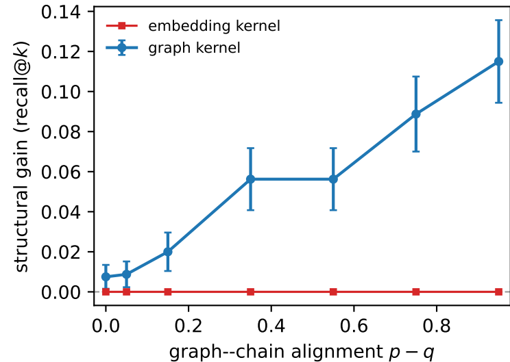
(A) Theorem: gain \propto alignment
