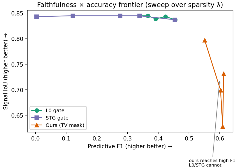
Figure 4: Faithfulness–accuracy frontier as the sparsity weight is varied (TV on). Sparsity-only gates occupy the high-IoU, low-F1 region; our TV mask occupies the high-F1 region they cannot reach, at strong signal IoU and zero distractor overlap.
