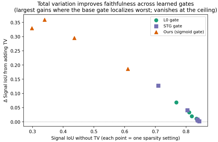
Figure 3: The total-variation penalty as a modular faithfulness prior. Each point is one sparsity setting of one gate; the vertical axis is the change in signal IoU from adding TV. Every point lies at or above zero (TV never hurts faithfulness), and the three gates ( L_0 , STG, and ours) fall on a common curve: the gain is largest where the base gate localizes worst and vanishes once it already saturates the IoU ceiling.
