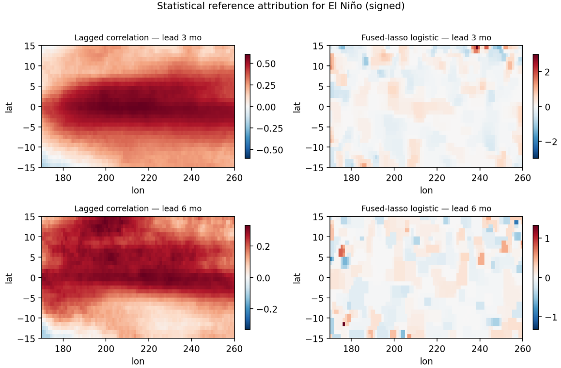
Figure 5: Statistical reference attribution for El Niño (signed). The lagged-correlation map (left) cleanly recovers the equatorial signal; the multivariate fused-lasso logistic (right) is destabilized by collinearity among the highly correlated equatorial cells.
