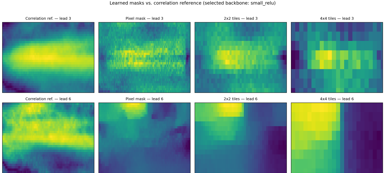
Figure 6: Learned input masks (pixel, 2 \times 2 , 4 \times 4 ) from the selected backbone beside the correlation reference at leads 3 and 6. At lead 3 the masks concentrate on the equatorial band that the reference identifies; at lead 6 they show a consistent off-equatorial emphasis.
