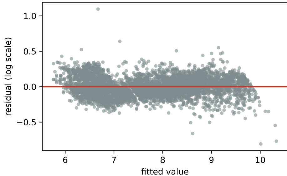
log(price) on log(carat)
