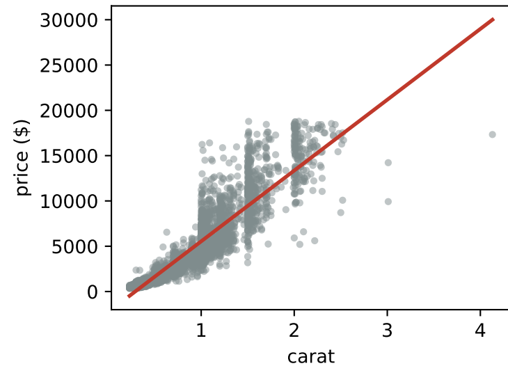
a straight line
