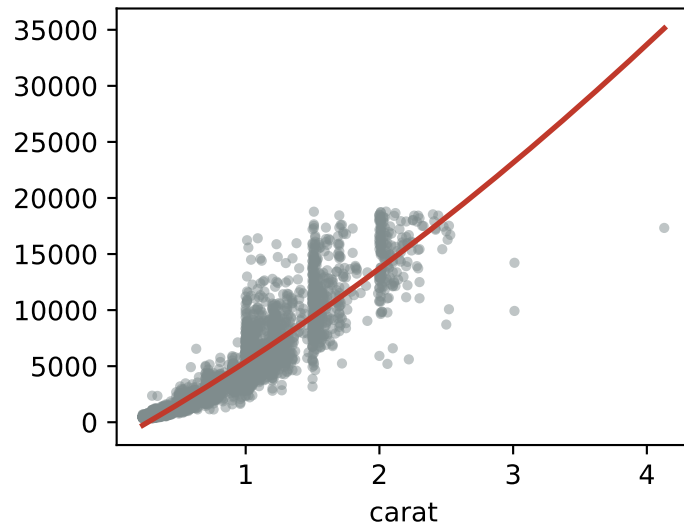
add a squared term
