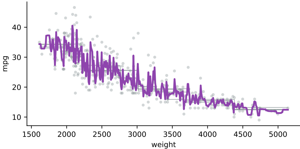
four single trees (thin) and their average (thick)
