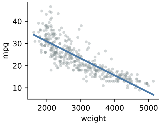
a straight line
