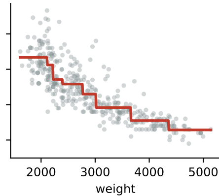
a tree (steps)
