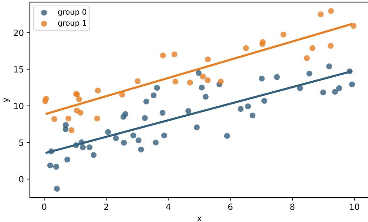
A 0/1 predictor shifts the line up (same slope)
