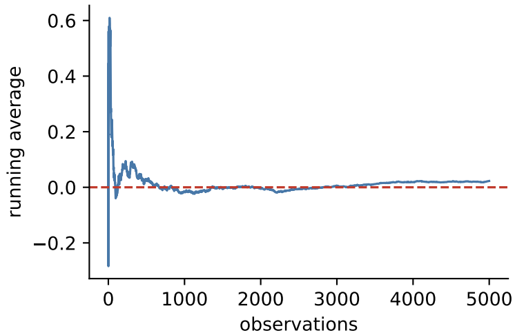
Well-behaved: the average settles
