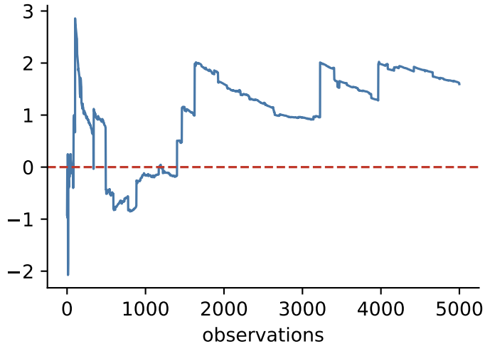
Heavy tail: it never does
