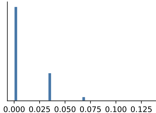
one in a hundred means of n = 30
