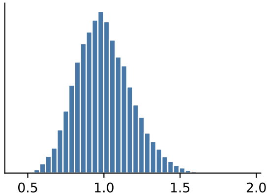
mildly skewed means of n = 30
