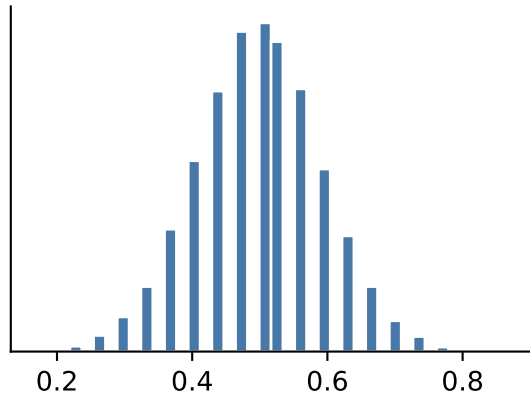
coin flips (0/1) means of n = 30
