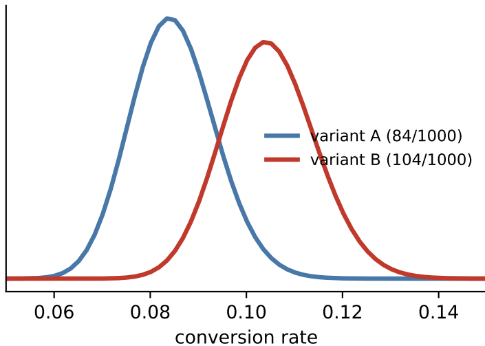
Two posteriors
