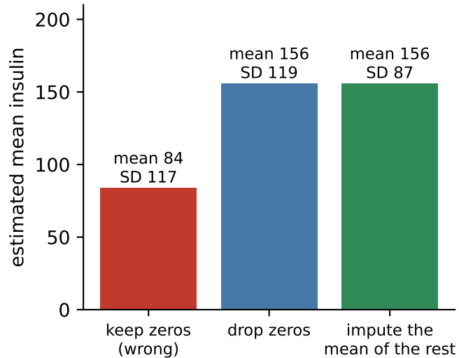
Three answers from one column
