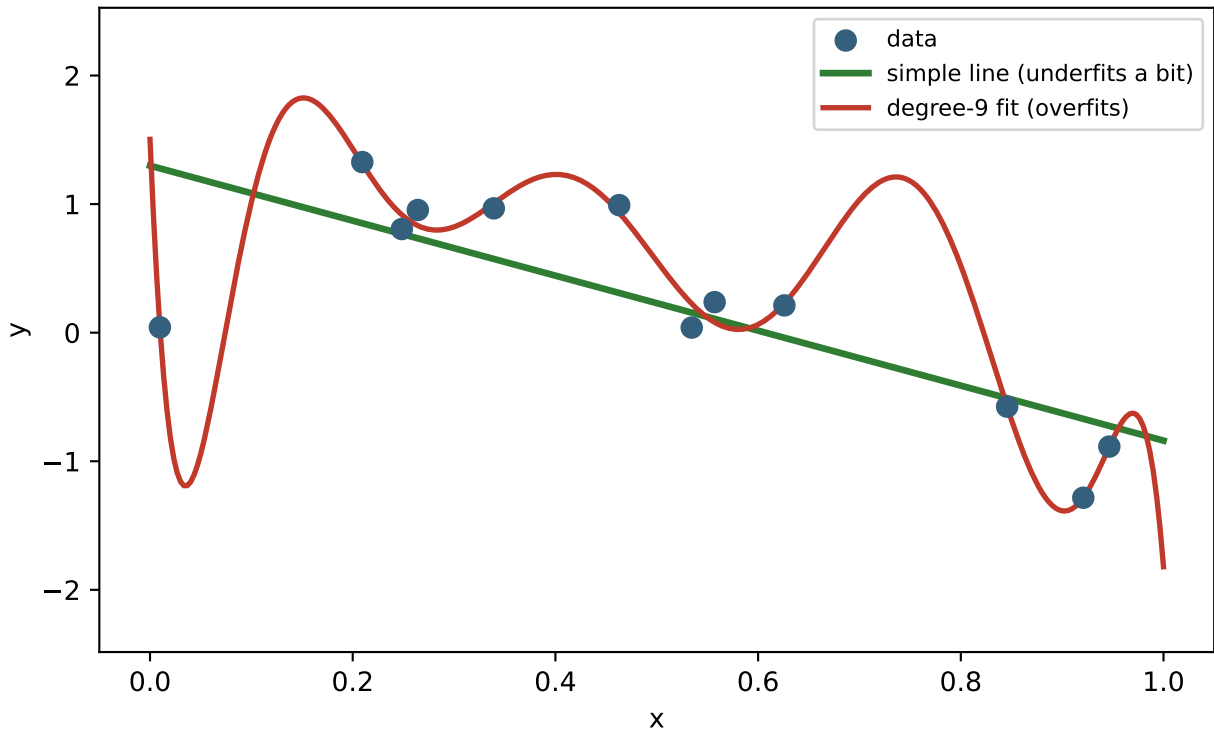
The wiggly curve nails the dots and learns the noise
