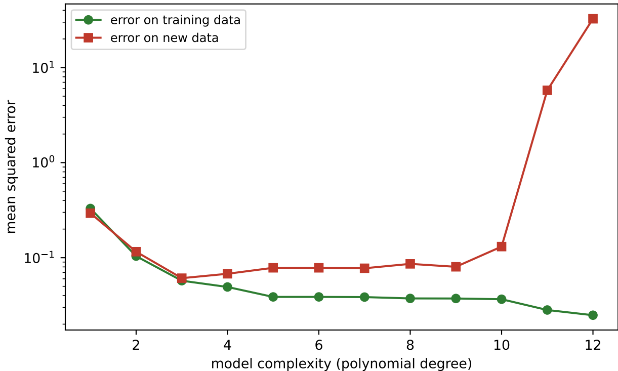
Training error keeps dropping; new-data error turns back up
