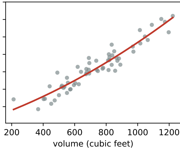
about right (polynomial degree 2)
