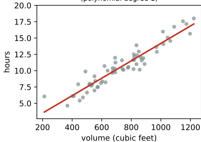
too simple (polynomial degree 1)
