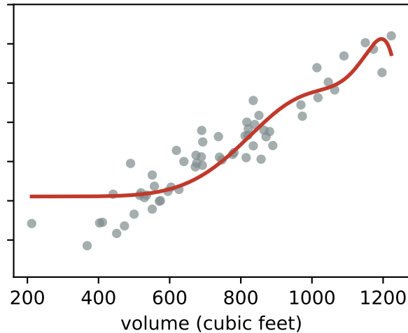
too flexible (polynomial degree 14)
