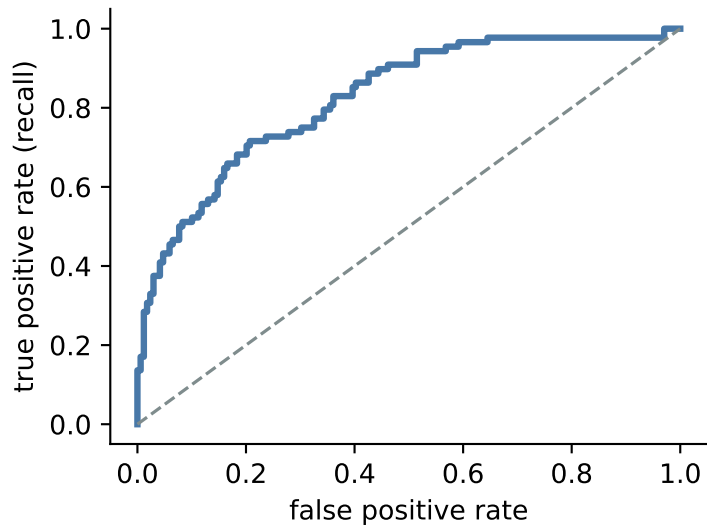
ROC curve, AUC = 0.83
